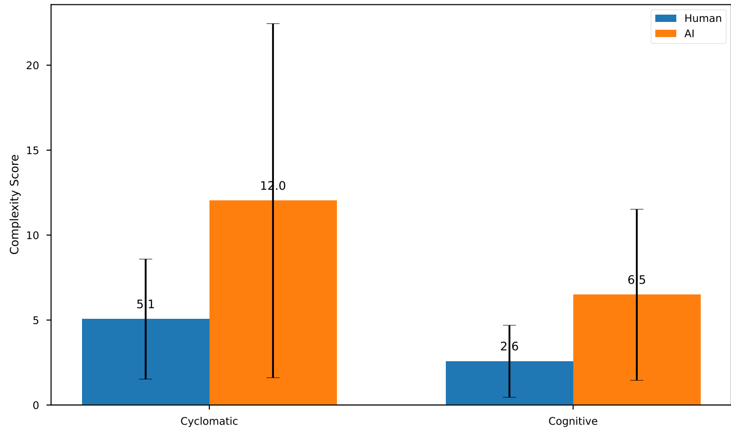
Code Complexity Comparison: AI vs Human
